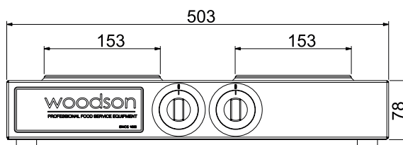
Front View Double
