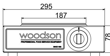
Front View Single
