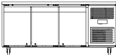
3 x Solid Doors AXR.UCGN.3 1795 x 700 x 840
