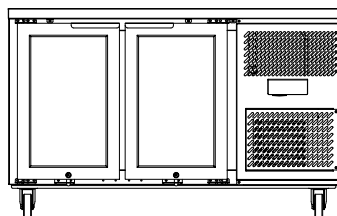
2 x Glass Doors AXR.UCGN.2G 1360 x 700 x 840
