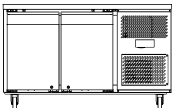
2 x Solid Doors AXR.UCGN.2 1360 x 700 x 840
