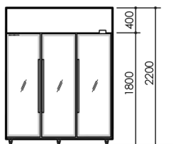
Integral front elevation
